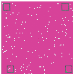
TE (both)
