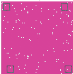
Go-Explore
