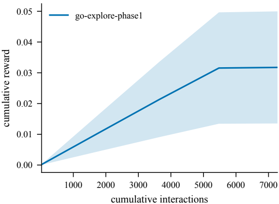
Reward accumulated over the evaluation budget
