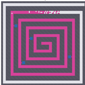
Go-Explore
