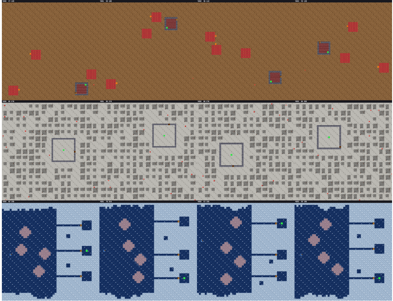
Figure 13: The hold-out ( test ) split, part 9 of 9: four instances of each family at seeds 4000–4003 with size-scaled placement jitter. Each panel is labelled with its seed, turn-aware optimal d^* , and horizon. Instances differ while the family’s arrangement holds — and the d^* values along a row show the difficulty distribution the split is drawn from.
