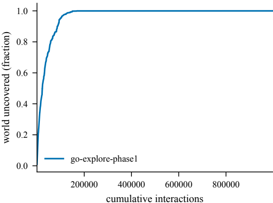
Cumulative coverage -- ClownChase
