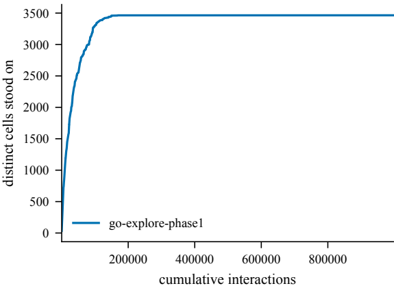
States discovered -- ClownChase
