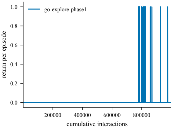
Return -- EpicChase8-120
