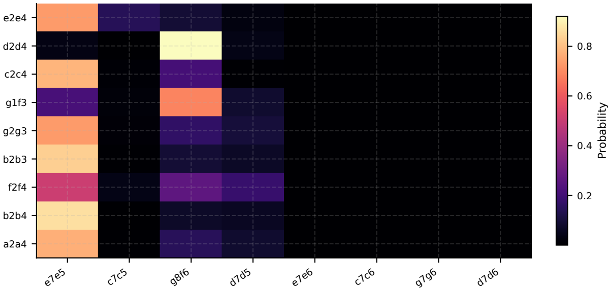
carlsen: SFT+DPO-V2 (w=0.1, \tau=0.75 ) opening reply matrix
