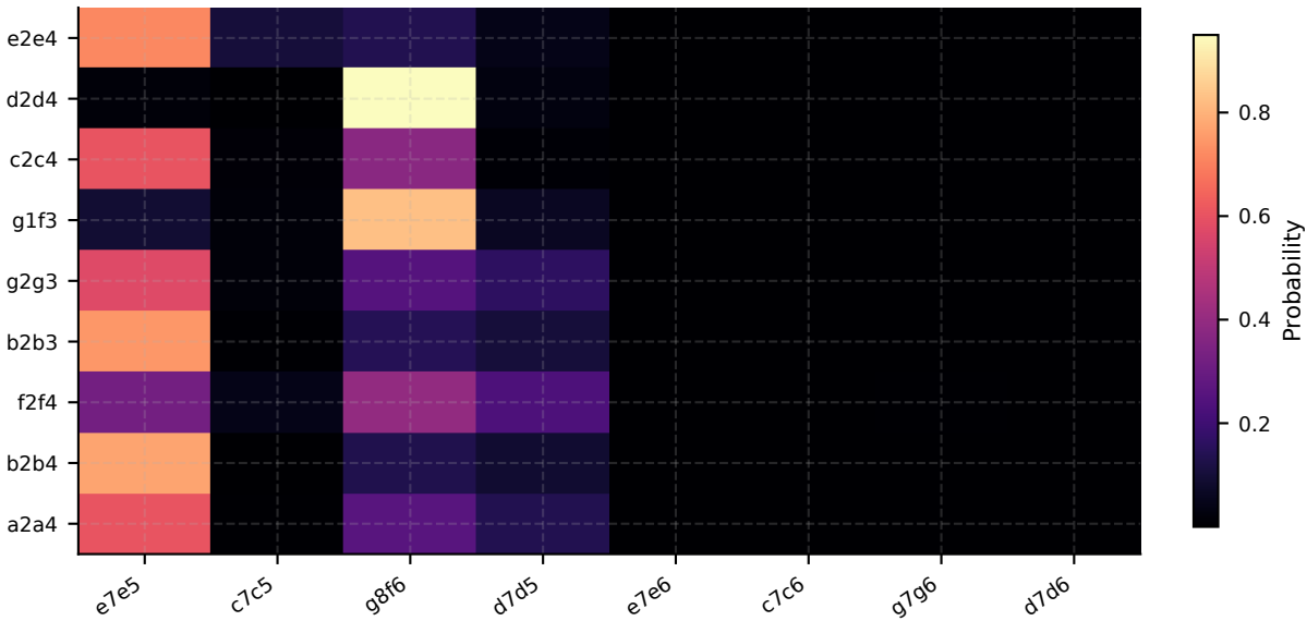
carlsen: SFT+DPO-V2 (w=0.1, \tau=1.25 ) opening reply matrix
