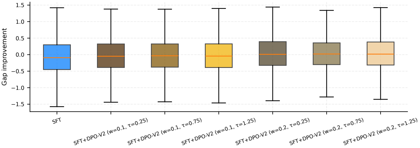
carlsen: distribution of gap improvement
