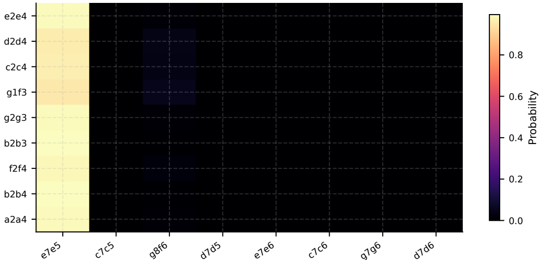
caruana: DPO-Beta=0.10 opening reply matrix
