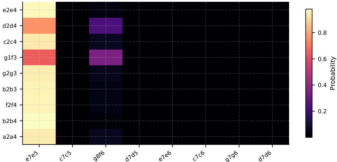
caruana: DPO-Beta=0.20 opening reply matrix
