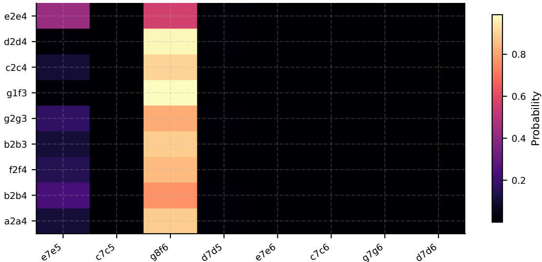
caruana: DPO-Beta=0.60 opening reply matrix
