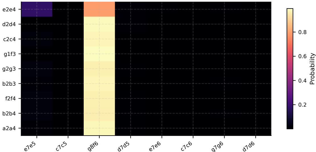
caruana: DPO-Beta=1.20 opening reply matrix
