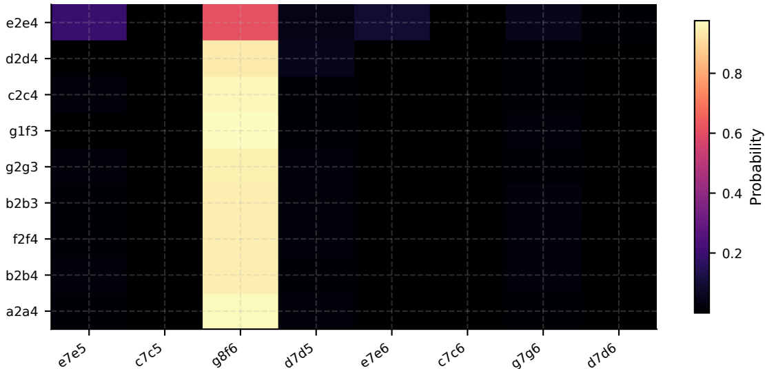
caruana: DPO-Beta=1.40 opening reply matrix
