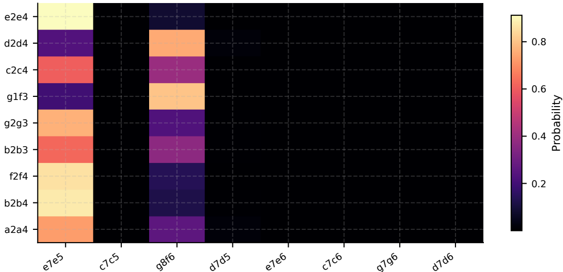
caruana: DPO-W-Margin-Beta=0.40-Gamma=0.50 opening reply matrix
