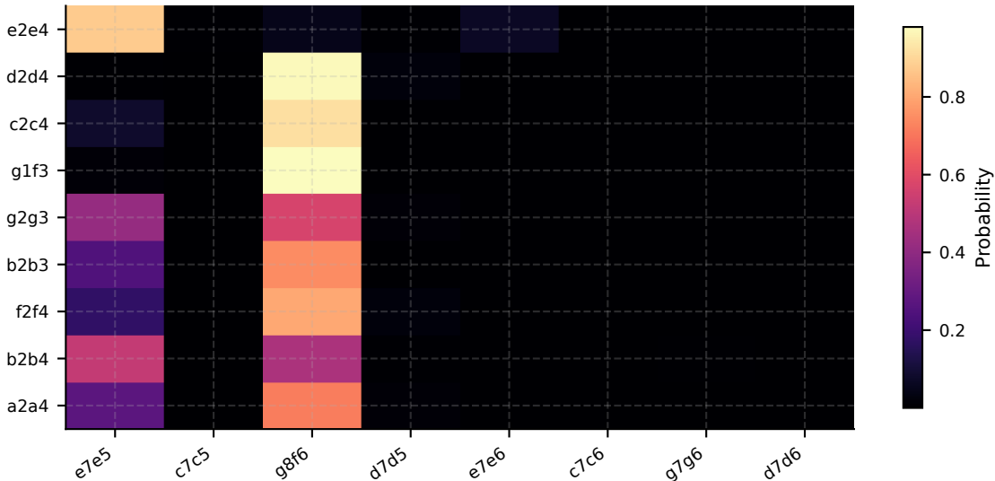
caruana: Kpo-Beta=0.40-Gamma=0.50 opening reply matrix
