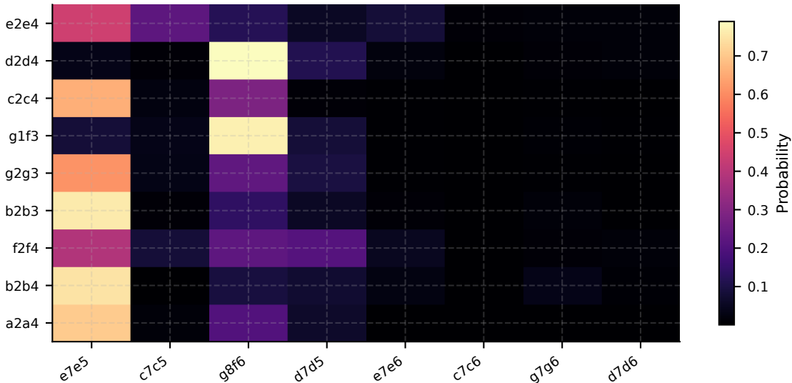
caruana: SFT-And-DPO-Beta=0.60-DPO-Loss-Weight=0.02 opening reply matrix
