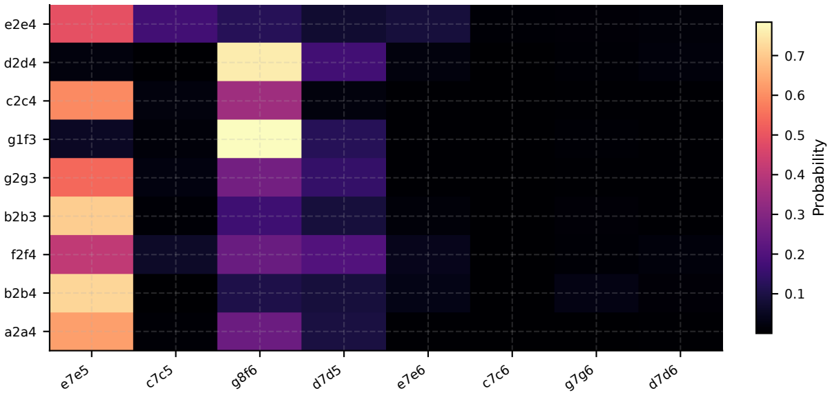
caruana: SFT+DPO-V2 ( w=0.2 , \tau=0.25 ) opening reply matrix
