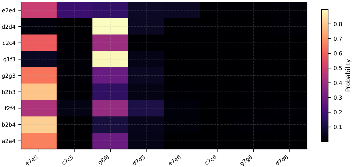
caruana: SFT+DPO-V2 ( w=0.2 , \tau=0.75 ) opening reply matrix
