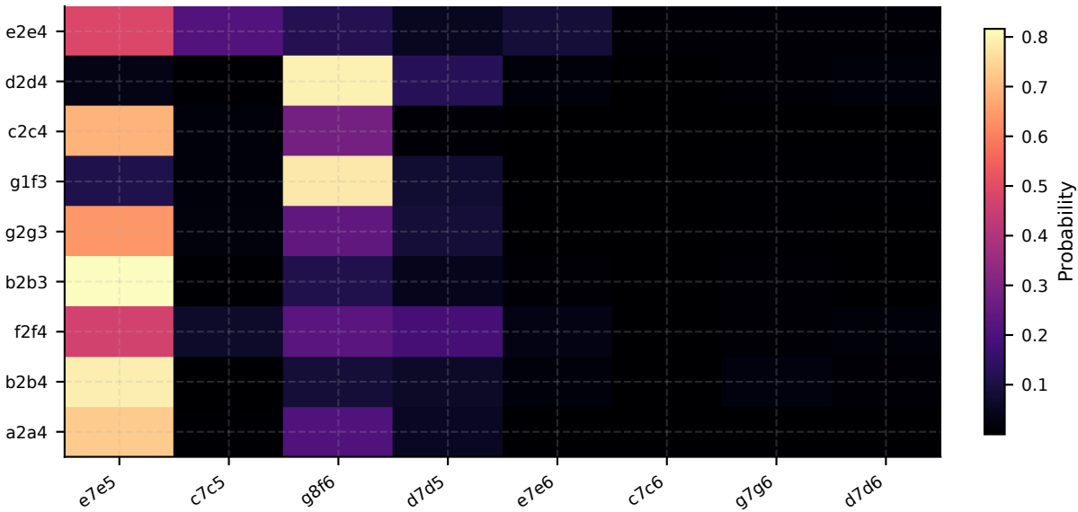
caruana: SFT+DPO-V2 (w=0.2, \tau=1.25 ) opening reply matrix
