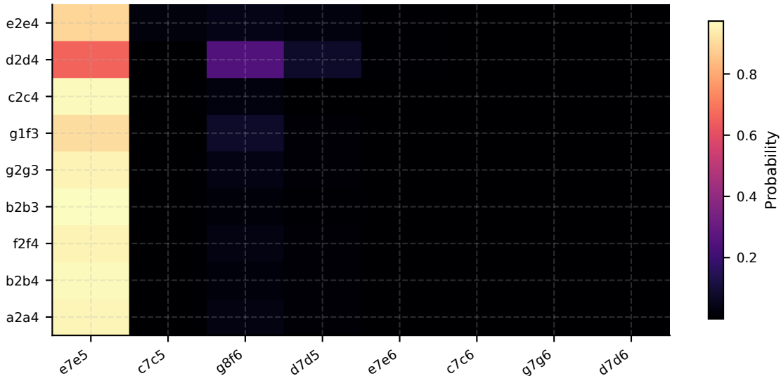
caruana: SFT-Pairwise opening reply matrix
