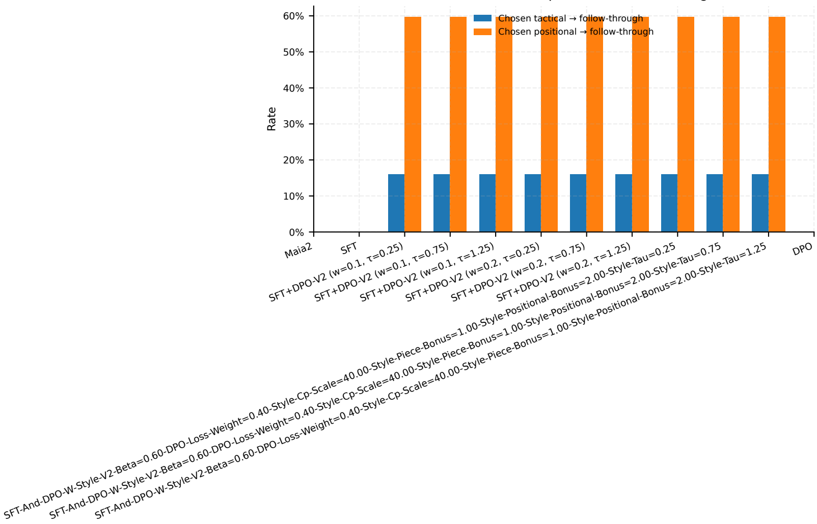
caruana: tactical vs positional follow-through
