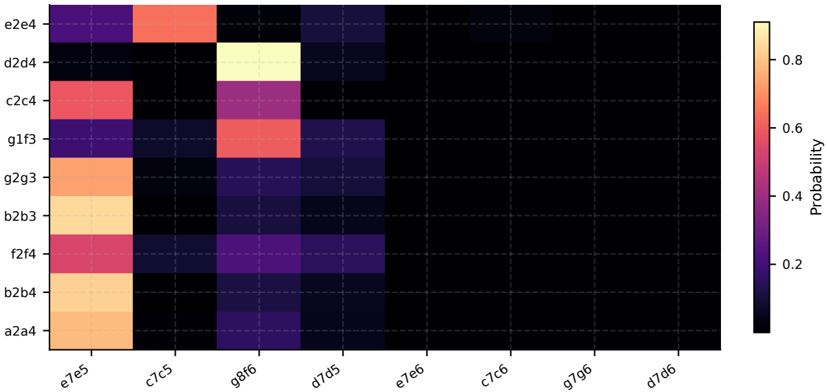
firouzja: SFT opening reply matrix
