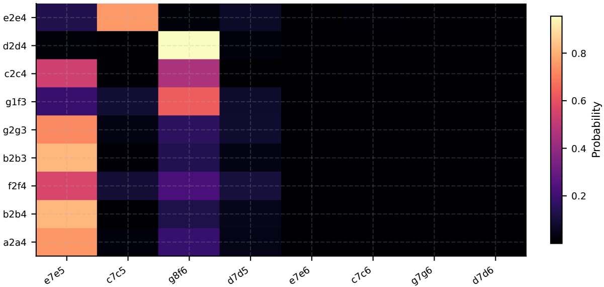
firouzja: SFT+DPO-V2 ( w=0.1 , \tau=1.25 ) opening reply matrix
