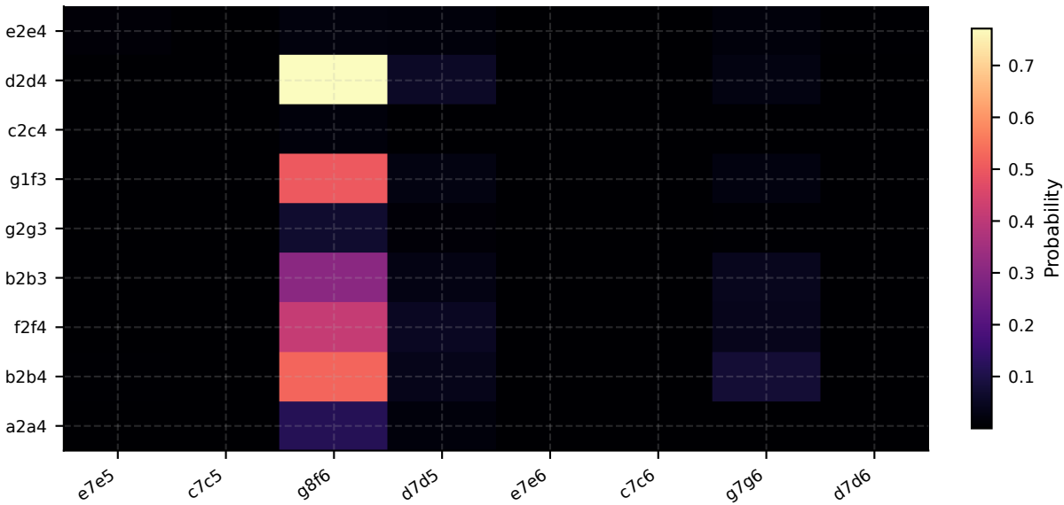
nakamura: DPO ( \beta=0.60 ) opening reply matrix
