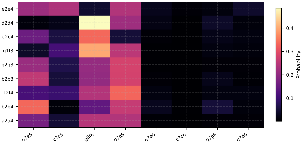
nakamura: SFT+DPO-V1 (w=0.1, \tau=0.25 ) opening reply matrix
