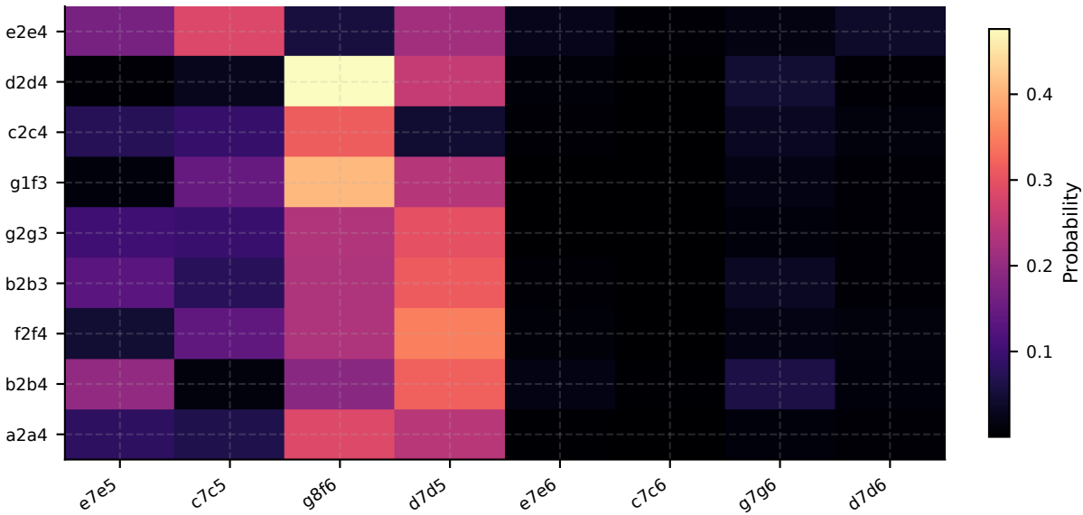
nakamura: SFT+DPO-V2 (w=0.1, \tau=0.25 ) opening reply matrix
