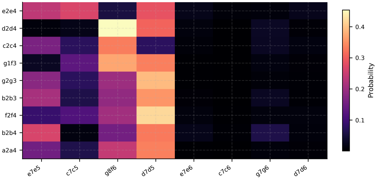
nakamura: SFT+DPO-V2 (w=0.1, \tau=1.25 ) opening reply matrix
