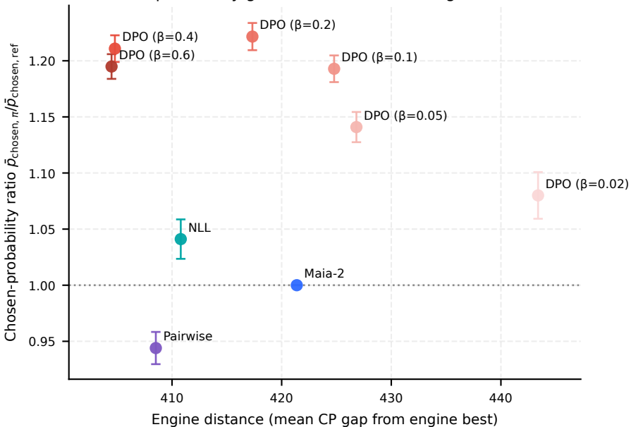
Chosen-move probability gain vs Distance from engine-best move (CP)
