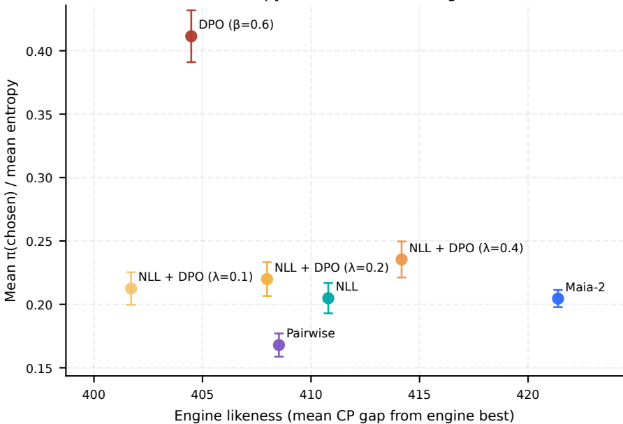
Mean \pi(\text{chosen}) / entropy vs Distance from engine-best move (CP)
