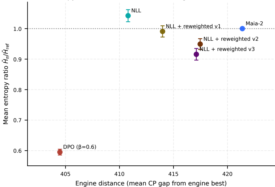
Entropy retention vs Distance from engine-best move (CP)
