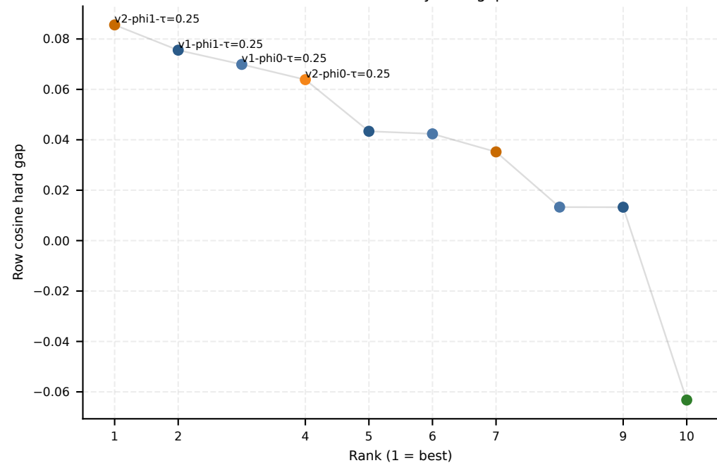
All runs ranked by hard gap
