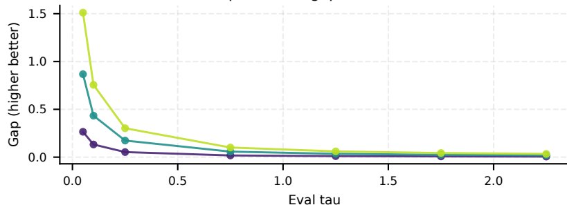
v2-phi0: Hard gap vs eval tau
