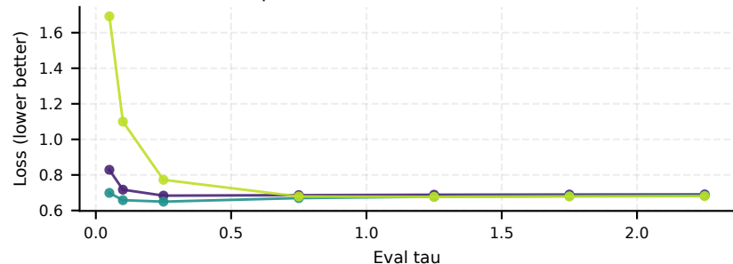
v2-phi0: InfoNCE-like loss vs eval tau
