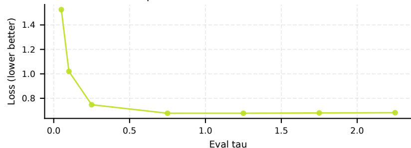
v2-phi1: InfoNCE-like loss vs eval tau
