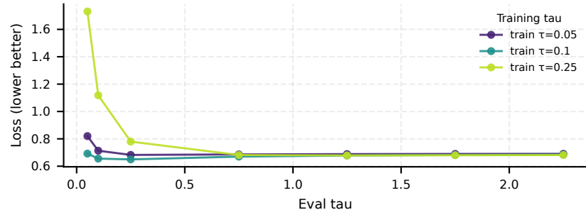
v1-phi1: InfoNCE-like loss vs eval tau
