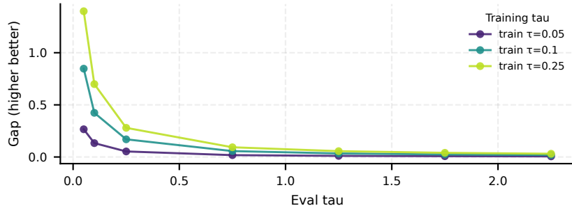
v1-phi1: Hard gap vs eval tau
