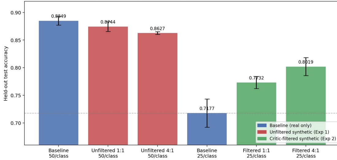
Figure 2 — Classification accuracy across all six conditions (mean \pm std, 5 seeds). Unfiltered augmentation degrades accuracy; critic-filtered augmentation improves it.
