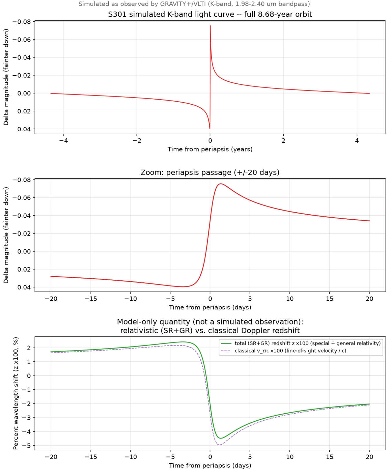
Figure 3. Simulated relativistic K -band light curve of S301 over one orbit (top), the periaapsis passage (middle), and the relativistic and classical spectral shifts near periaapsis (bottom). The lower panels show a generic passage in time from periaapsis; precession changes only the orbit's orientation on the sky, so the shape is the same for either real passage. The bottom panel is a model-internal quantity (SR: special-relativistic Doppler shift; GR: gravitational redshift) that explains the magnitude curves above it; no instrument in this campaign measures a spectral shift.
