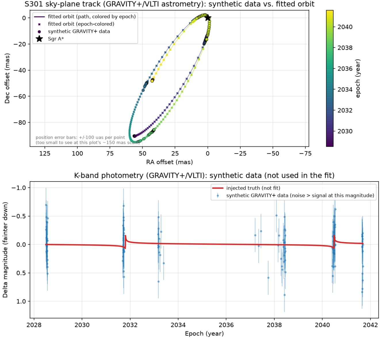
Figure 4. Top: fitted sky-plane track (GRAVITY+VLTI astrometry) vs. synthetic data, epoch-colored, showing the precessing orbit’s two passages. Bottom: simulated K -band photometry vs. the injected truth curve (not used in the fit). An animated version ( s301_precession.mp4 , included as an ancillary file with this submission and available at https://github.com/jcatanza/s301-schwarzschild-precession/blob/master/output/s301_precession.mp4 ) extrapolates the same real 1PN precession rate over 20 orbits ( \sim 174 yr) to make the rosette pattern visible; only the two orbits actually analyzed in this paper are highlighted there, and the extrapolation is labeled explicitly on-screen throughout.
