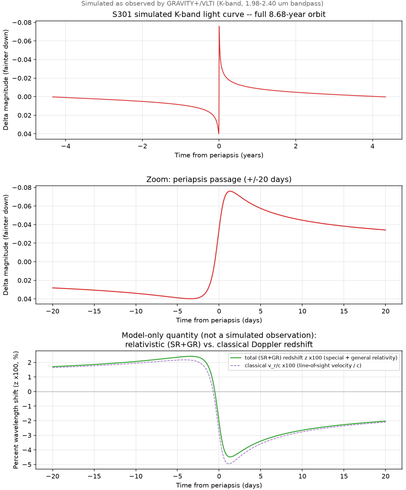
Figure 3. Simulated relativistic K -band light curve of S301 over one orbit (top), a zoom on the periaapsis passage (middle), and the relativistic vs. classical spectral shift near periaapsis (bottom). The middle and bottom panels show a generic passage, in time measured from periaapsis itself; the shape is the same for either real passage (2031.8 or 2040.5), since precession changes the orbit’s orientation on the sky, not its brightness or redshift as a function of time from periaapsis. The bottom panel is a theoretical, model-internal quantity (SR = special-relativistic Doppler shift, GR = Schwarzschild gravitational redshift), not a simulated observation: no instrument in this campaign measures a spectral shift directly (Section 3.2); it is shown to explain what drives the delta-magnitude curves above it.
