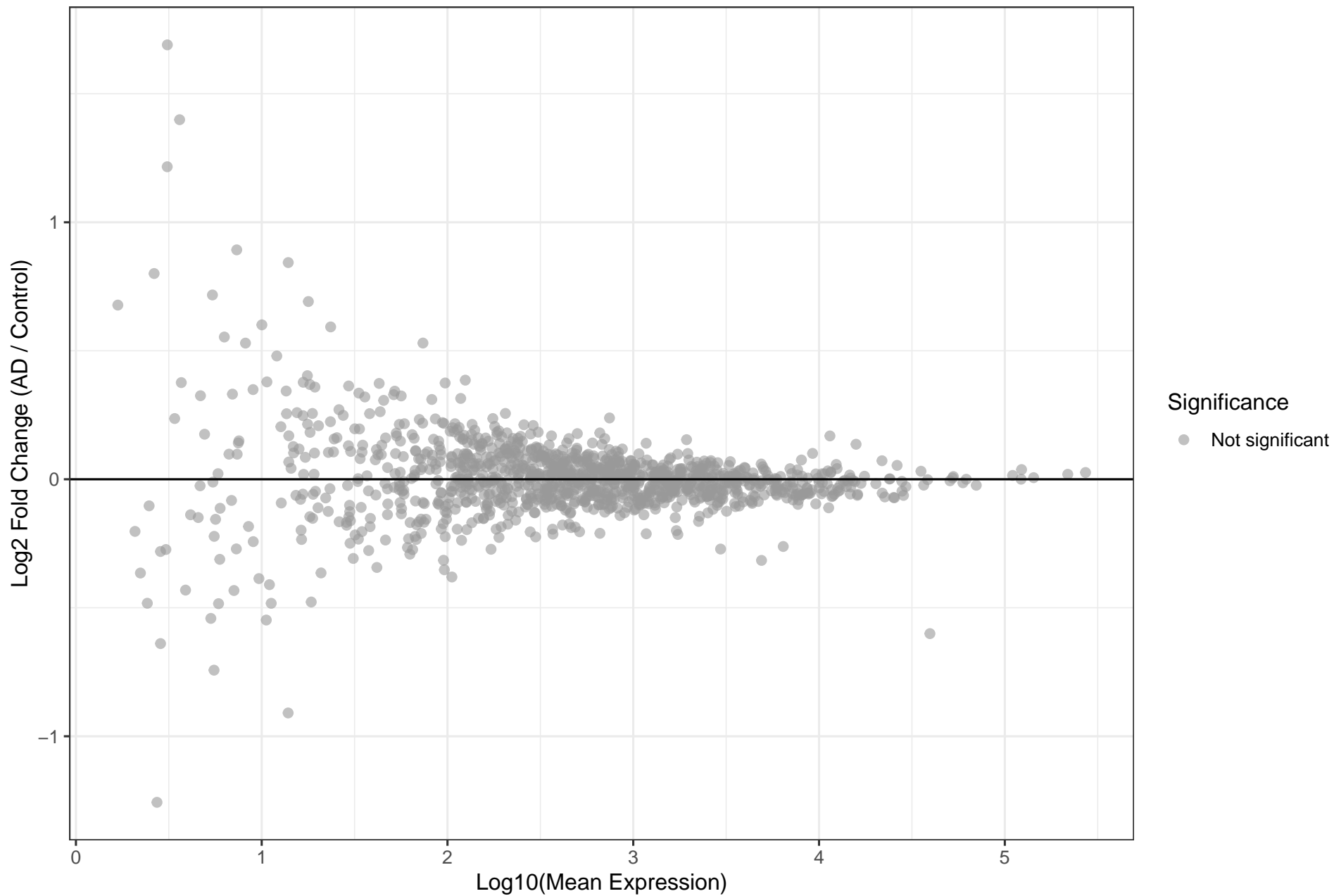
MA Plot: TE Expression (AD vs Control)
