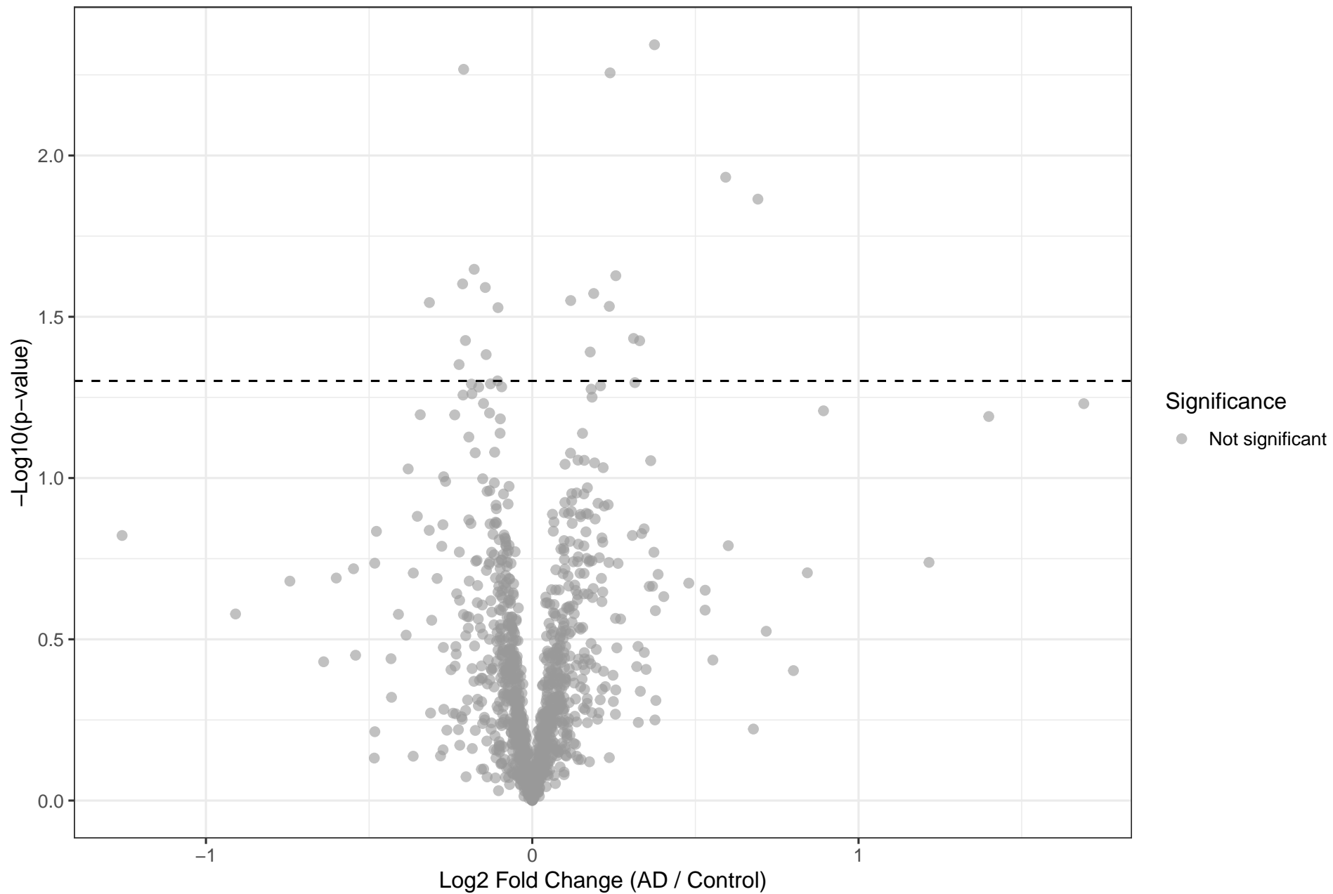
TE Differential Expression: AD vs Control
