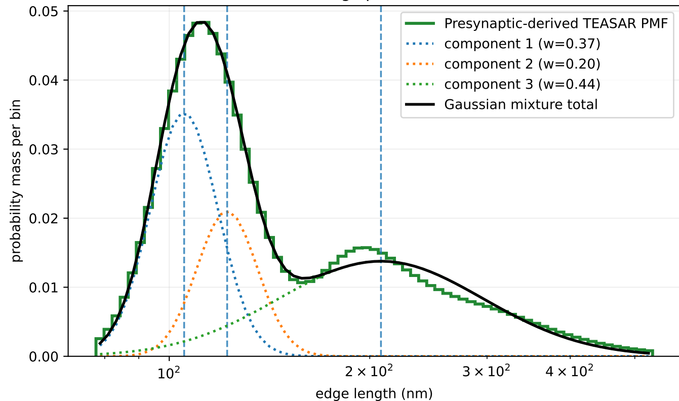
Presynaptic-derived TEASAR: components with >5 presynaptic sites Log-space fit
