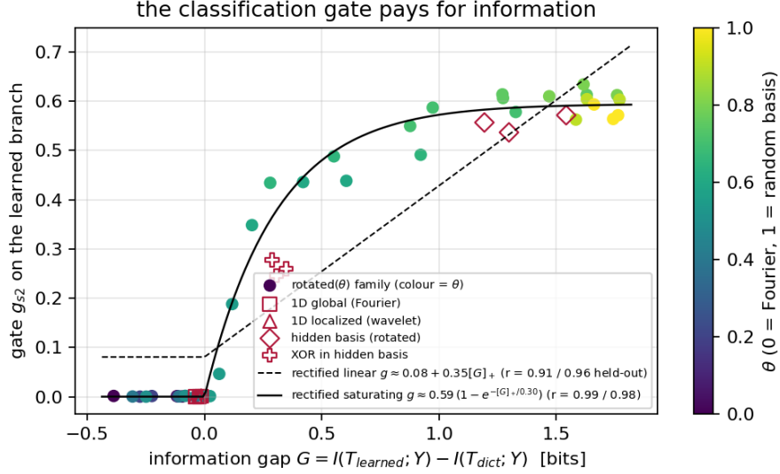
Figure 4: The classification gate against the information gap. Filled circles: the rotated family, coloured by \theta ; open markers: the four tasks of [?], not used in the fit. Solid: the gate law, Equation (??); dashed: the rectified line.
