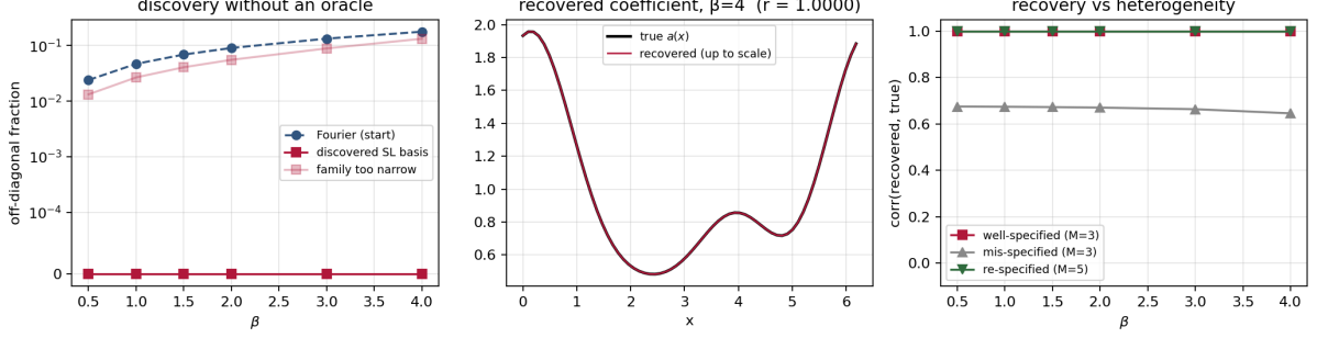
Figure 7: Discovering the basis. Left: the discovered SturmLiouville basis diagonalizes as well as the oracle, with no oracle; the pale curve is the same search with a family too narrow to contain the truth. Centre: the recovered coefficient over the true one. Right: recovery against heterogeneity for well-specified, mis-specified and re-specified families.
