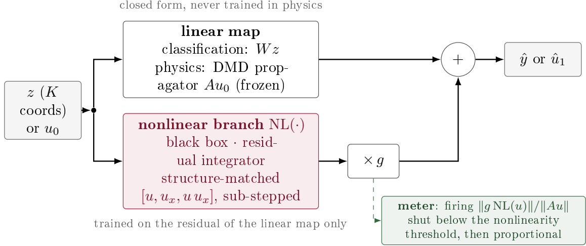
Figure 3: Zoom on Stage 3, the predictor. In physics the linear map is the closed-form DMD propagator, frozen; only the gated branch trains, on the residual.
