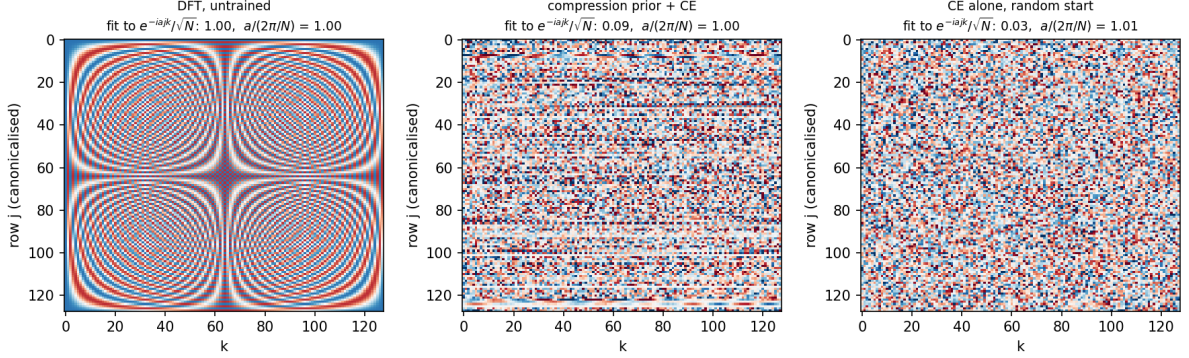
Figure 5: Real part of three unitaries after gauge canonicalisation, with the closed-form reading score. Left: the DFT reads exactly. Centre and right: task-trained bases do not.
