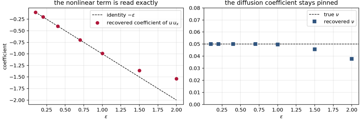
Figure 10: Reading the operator. Left: recovered coefficient of uu_x against the ground truth -\epsilon . Right: the linear (diffusion) coefficient stays pinned at \nu .
