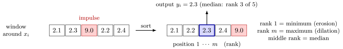
Figure 1: A rank filter. The window is sorted and one rank is selected. The impulse (9.0) is ignored.
