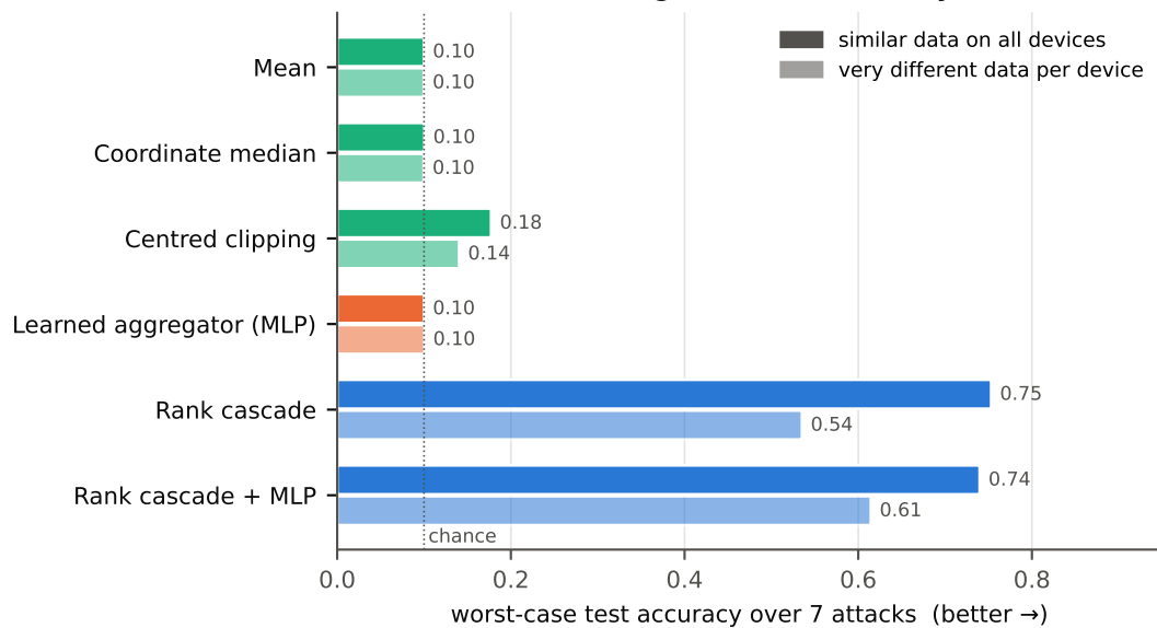
(b) Federated learning with 4 of 20 faulty devices
