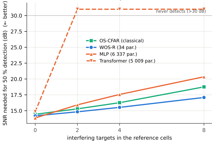
(a) Radar detection accuracy (correlated clutter)
