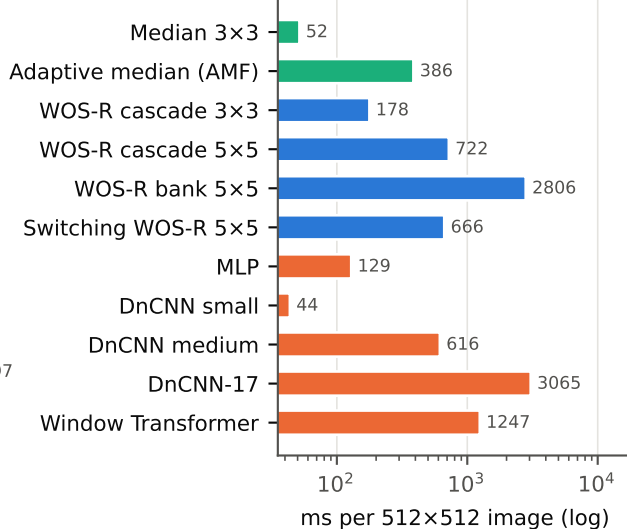
(c) Latency (PyTorch, 1 thread)
