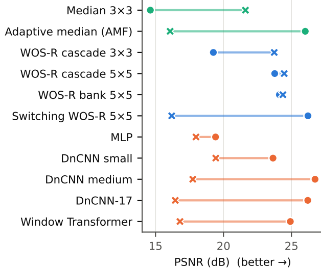
(a) Image quality, BSD68
