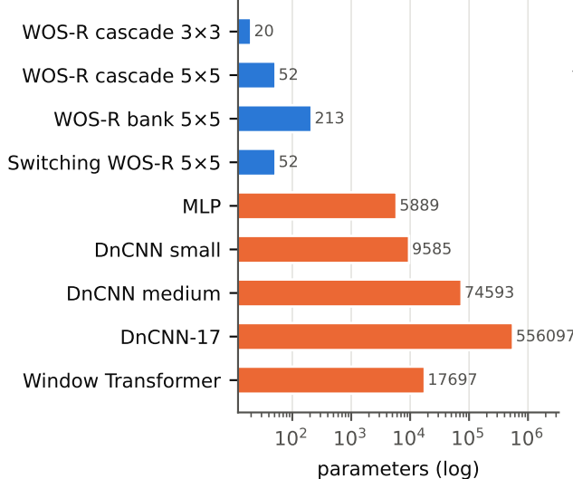
(b) Model size
