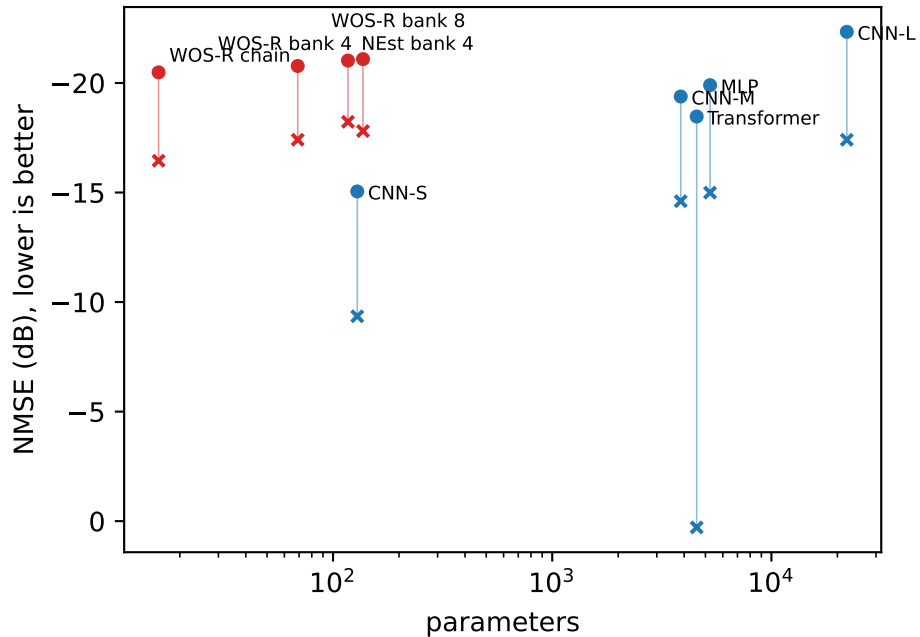
B1 1D impulsive: o in-distribution, x OOD amplitude x2
