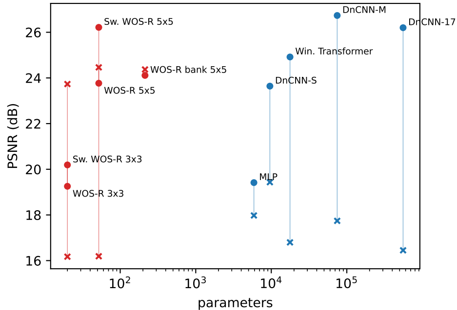
B3 BSD68: o SP 50%, x RVIN 40% (OOD)
