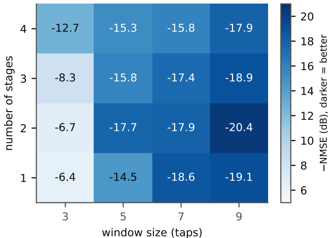
WOS-R cascade, 1D impulses (mean of 2 runs)
