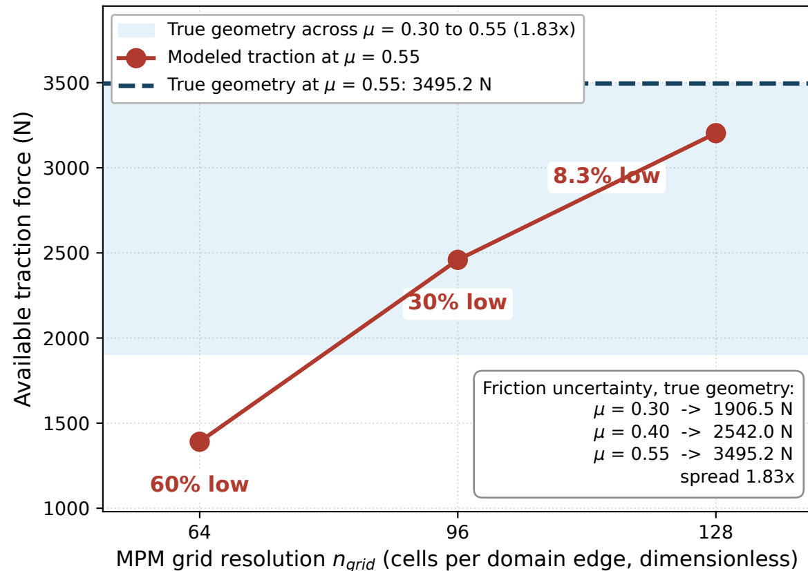
Tire traction at \mu = 0.55 , 1100 kg vehicle
