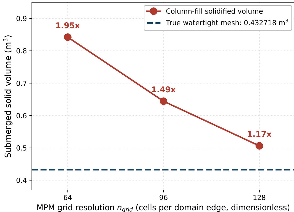
Solid volume below the 0.30 m waterline
