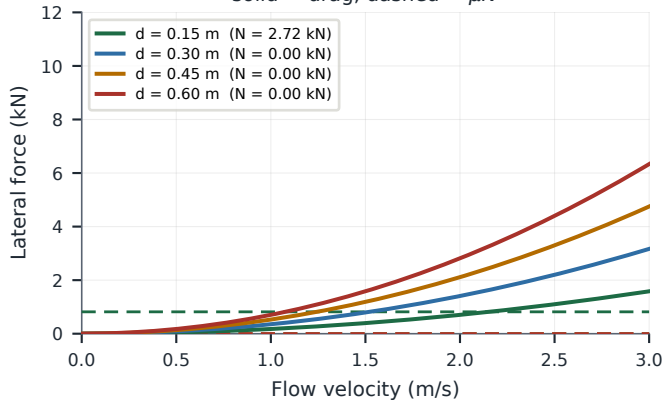
Drag vs. friction limit solid = drag, dashed = \mu N
