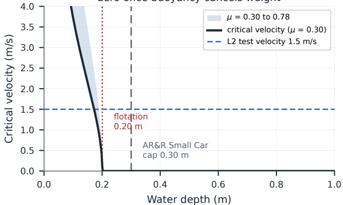
Critical velocity vs. depth zero once buoyancy cancels weight
