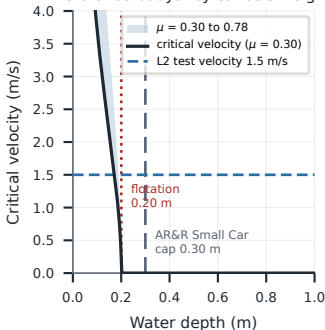
Critical velocity vs. depth zero once buoyancy cancels weight
