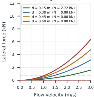
Drag vs. friction limit solid = drag, dashed = \mu N
