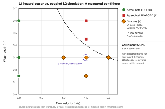
Fig. 5. L1 hazard scalar versus coupled L2 simulation, 9 measured conditions from data/l2_results_from_wandb.csv . Agreement holds at 5 of 9 (55.6%): 3 conditions where both agree FORD, 2 where both agree NO-FORD. All 4 disagreements run one way, L1 permits and L2 refuses, with no reverse cases in this dataset. One flagged cell (marked ‡) has an l1_haz_score that disagrees with its own D \times V product; the figure plots the consistent D \times V value throughout and the discrepancy is noted rather than silently resolved.
