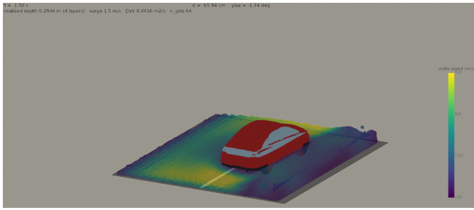
Fig. 7. One frame (45 of 90, t = 1.50 s) from run g64_m1100 of the same data/all_runs_inventory.csv inventory: the watertight Yaris hull carried at 1100 kg (AR&R small passenger), n_grid=64 , requested depth 0.30 m (realized 0.2944 m, four water layers), and inflow velocity 1.5 m/s, giving D \times V = 0.4416 \text{ m}^2/\text{s} . This is coupled-MPM solver output, not a Gaussian-splat reconstruction: the vehicle is the crash-validated finite-element hull carried as a rigid body, and the water surface is an isosurface reconstructed from the run’s own MPM particles, coloured by water speed. The vehicle is drawn as the full watertight mesh posed by the rigid-body transform, while the physics ran on the 8,905 material points filling that hull. It is included to make the coupled simulation legible as a physical scene, not as a validated result. This run is one of the 7 of 17 that exceed the 10% particle-passthrough gate, at 10.7%, and the frame is mid-run, so the displacement printed in the frame is not the run’s final reported value.
